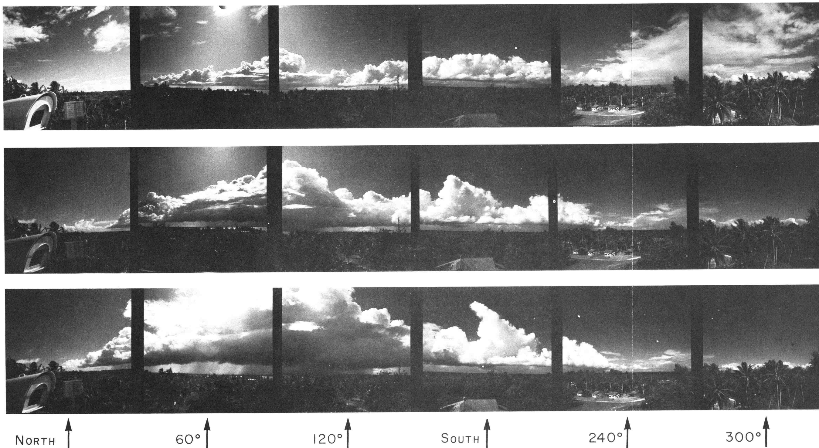
Fig. 48 Example of routine panoramic cloud photography accomplished during the Line Islands Experiment. This view is from the photo tower on Fanning on 19 April, at 1900, 1920 and 1930 GMT, top to bottom, or 1 hr prior to the ATS-1 photograph of Fig. 35. The "birdhouse" shelters the Bolex cine camera. With relatively minor exceptions (see Section IV), similar panoramas were taken every daylight hour of every day from Palmyra, Fanning, Christmas and the USC&GSS Surveyor . (NCAR photo)
