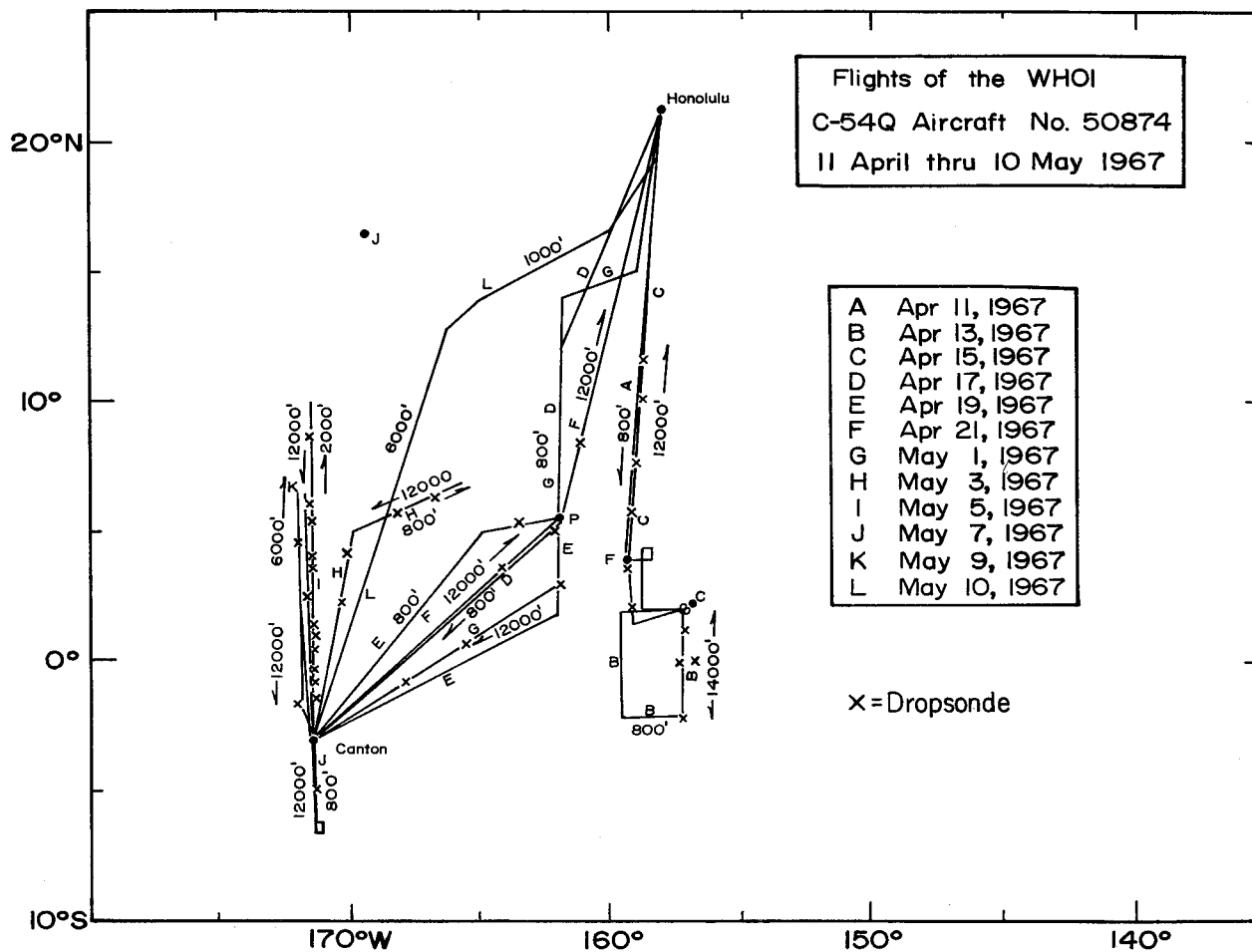
Fig. 33 Map showing tracks flown by the Woods Hole Oceanographic Institution C-54Q aircraft during the Line Islands program. The black dots identified as J, P, F and C refer to Johnston, Palmyra, Fanning and Christmas Islands, respectively.
