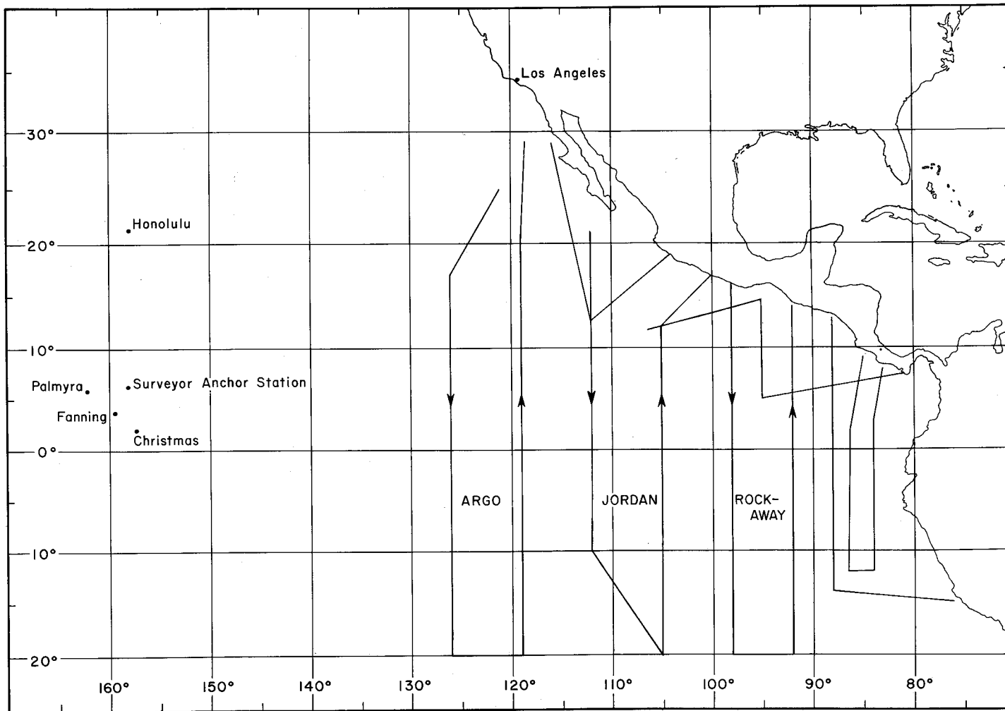
Fig. 36 Major ship tracks of the EASTROPAC program during the period of the Line Islands Experiment. The ships which are identified by name obtained upper air data.
