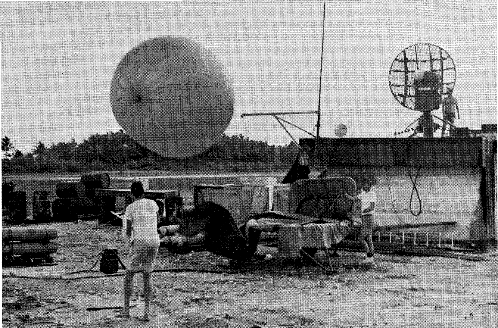
Fig. 9 GMD-1B release on Palmyra, looking northeast. (NCAR photo)
