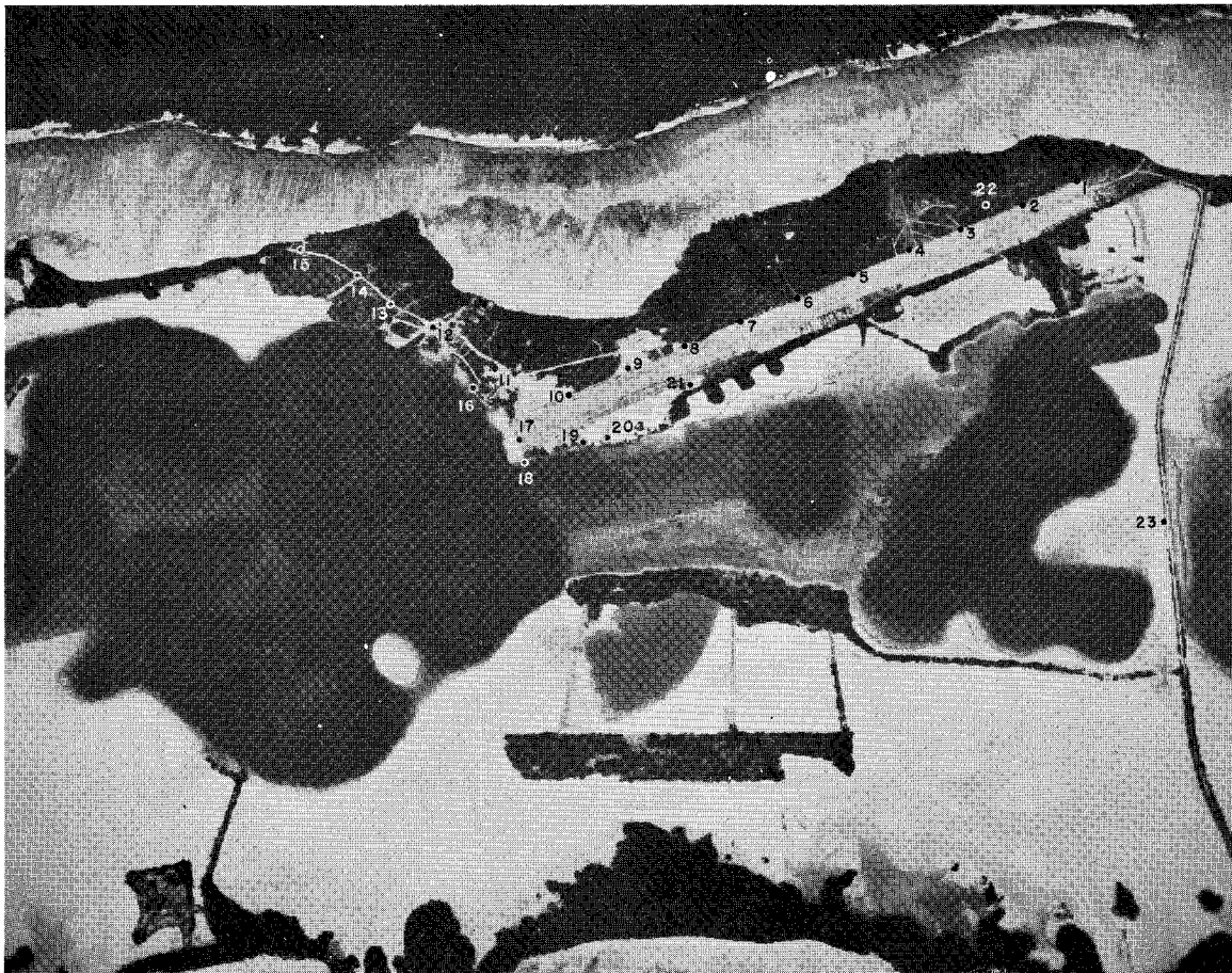
Fig. 3 Near-vertical aerial view of developed portion of Palmyra, taken from an altitude of 10,000 ft. The runway dimensions are 300 by 6,000 ft. It was cleared of heavy shrubbery in mid-February, 1967. The various observing facilities are located by number: (1-14) locations of rain gauges 1-14; (15) radar and photo tower; (16) second Bolex time-lapse camera, aimed toward west-southwest; (17) second Rolleiflex camera, forming stereo pair with camera on radar tower; (18) radiometer site; (19) U.S. Air Force GMD site; (20) U.S. Army surface site; (21) APT receiving site; (22) atmospheric electricity measurements site; (23) causeway site. (Photo by Bob Kendall)
