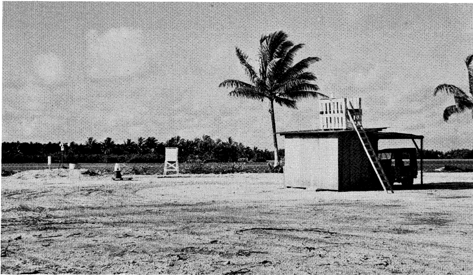
Fig. 5 U.S. Army surface observation site, Palmyra, showing (left to right) the MRI, Jardí and Dines rain gauges, instrument shelter, and observers' shelter. All brush was cleared from the area during the first week in March. To the east (left) of the instruments, the nearest palm tree is 400 ft distant. (NCAR photo)
