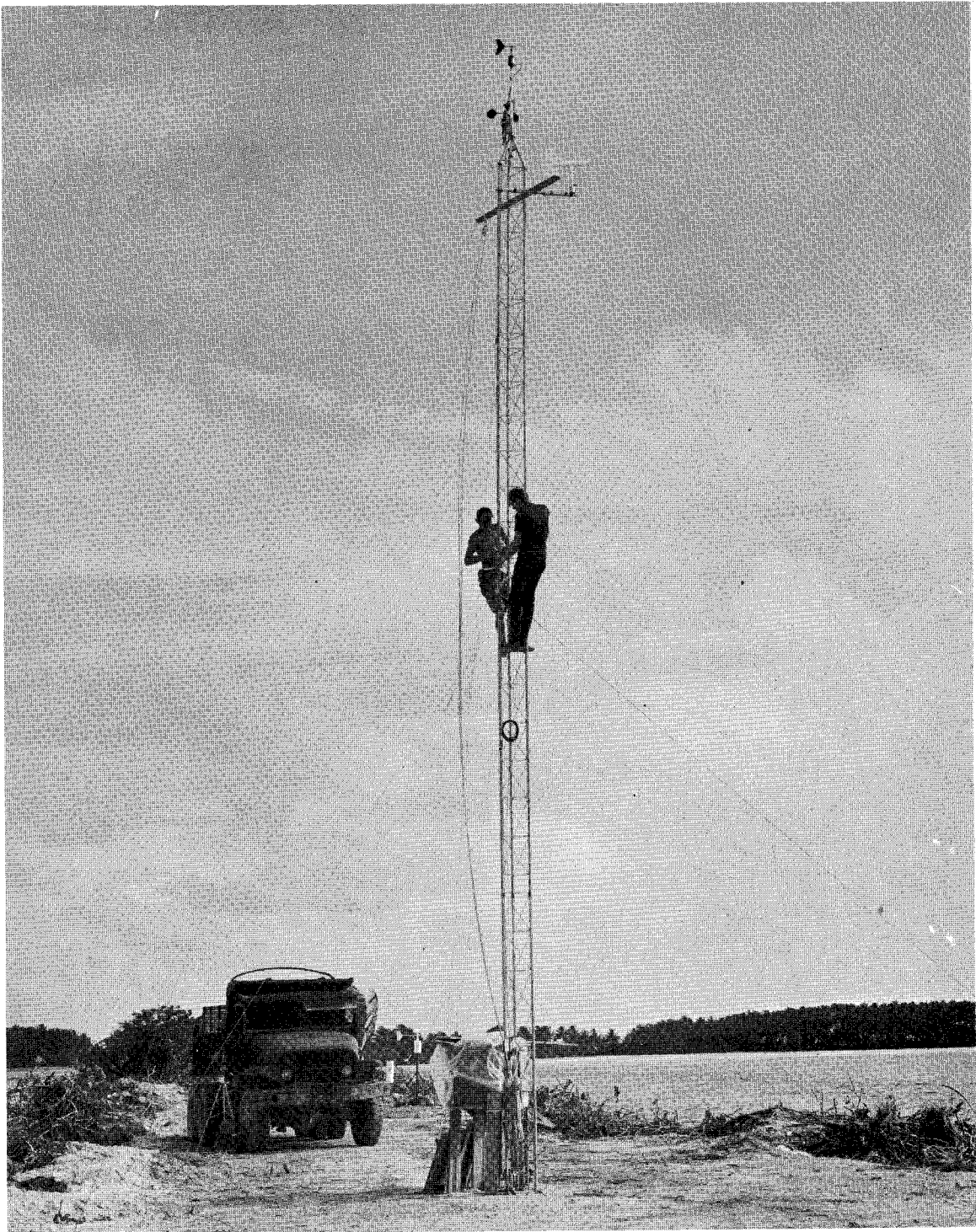
Fig. 7. Causeway site, Palmyra, looking north, showing the GMQ-12 wind sensors on a 40-ft tower, and the MRI of Fig. 6 in the background. (NCAR photo)
