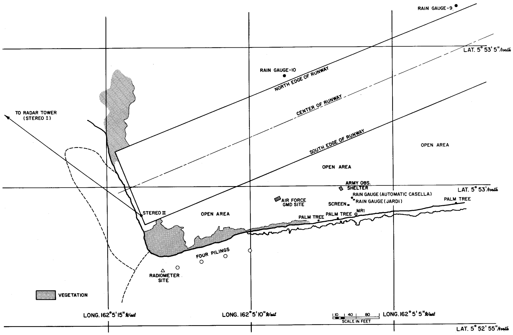
Fig. 4 Sketch of observing facilities near west end of runway, Palmyra. (Based on a survey by H. M. E. van de Boogaard and A. Pallmann)
