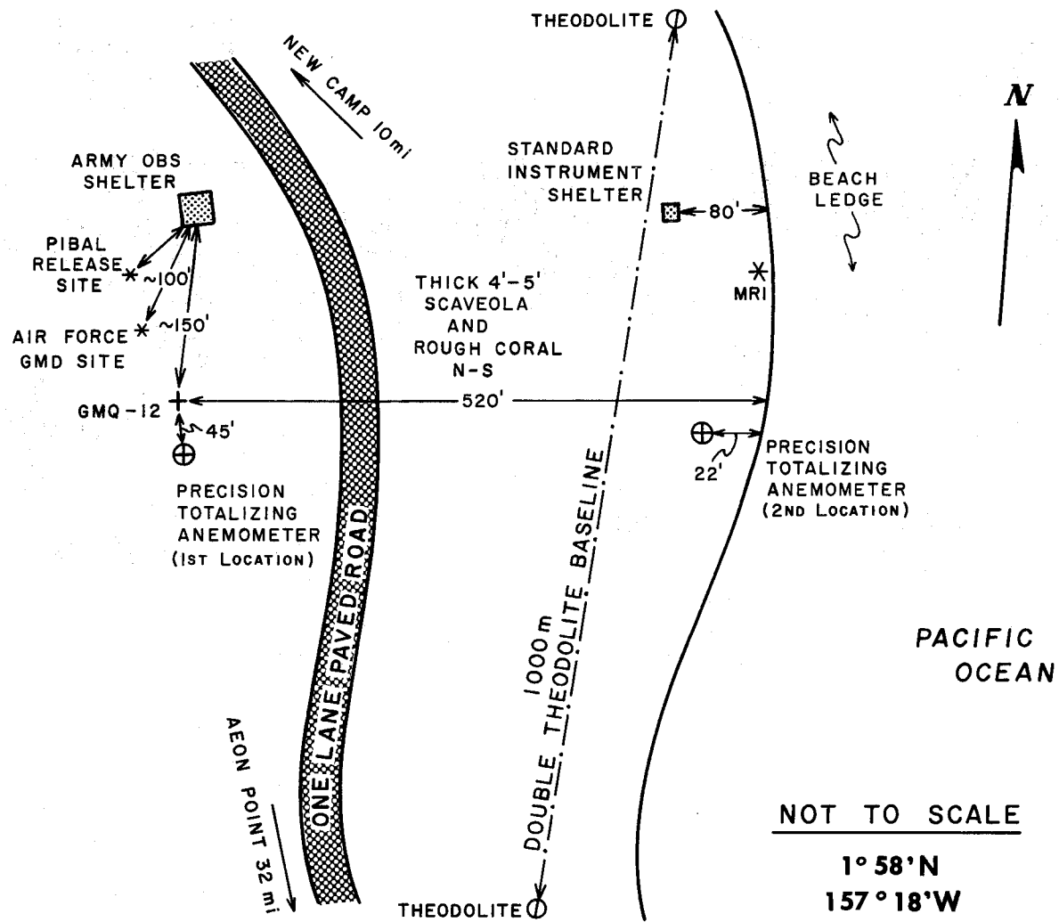
Fig. 22 Main observing area at Northeast Point, Christmas Island. (Based on sketch by Frank Harrison)
