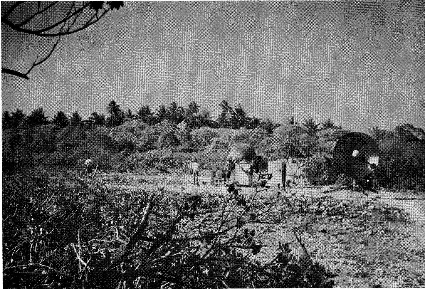
Fig. 18 Fanning Island rawin release site looking north-northeast. This area is devoid of palms but has considerable lower vegetation. Tracking antenna is on the far right, hydrogen generators just to the right of center. (NCAR photo)
