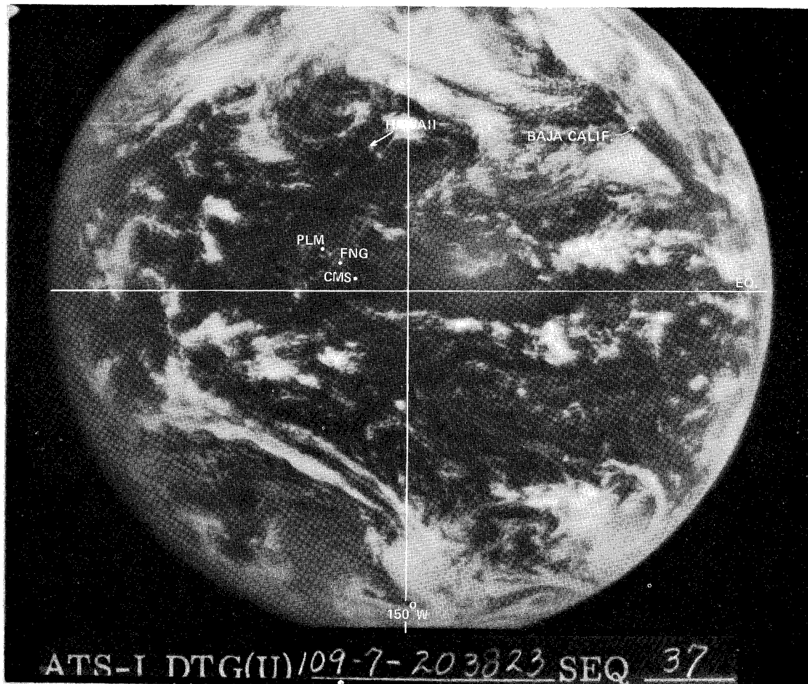
Fig. 35 Typical ATS-1 photograph taken during period of most intensive coverage. The legend identifies the day (109th day of the year -- 19 April), the year (1967), the time (203823 GMT), and the numerical sequence number (37th picture of the day).
