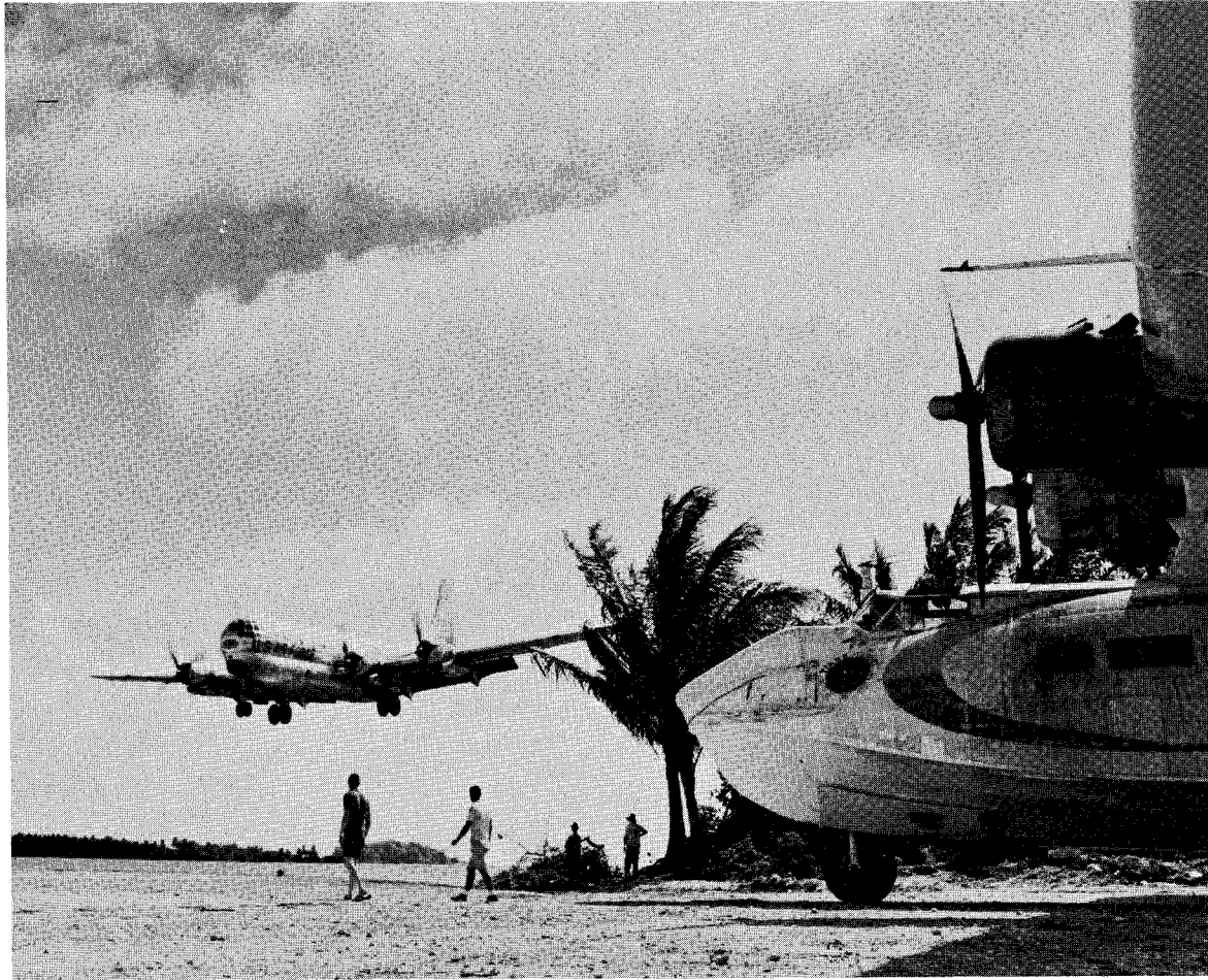
Fig. 46 The U.S. Air Force C-97 landing at Palmyra, with the PB4Y in the right foreground. These aircraft made weekly supply flights to Christmas and Palmyra. They were operated by the 146th MAW, Van Nuys, California, and supported by California, Arizona and Utah units of the Air National Guard. (NCAR photo)
