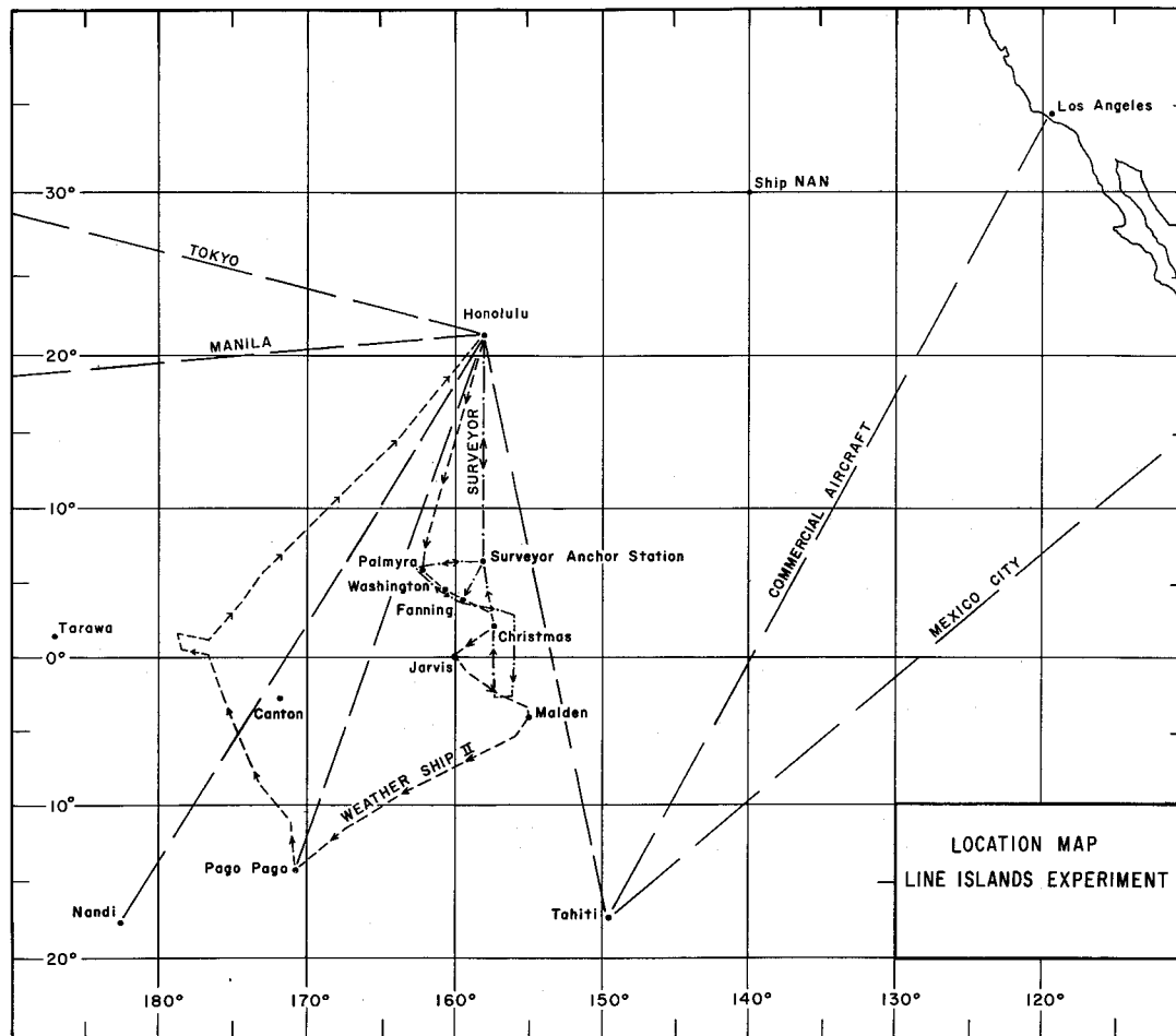
Fig. 1 Location map, Line Islands Experiment, showing tracks of the USC&GSS Surveyor and Weather Ship II , and commercial jet aircraft routes from which routine data are available. During the experimental period, the rawinsonde stations nearest the Line Islands were Honolulu, Canton Island, Nandi, Pago Pago and Tahiti.
