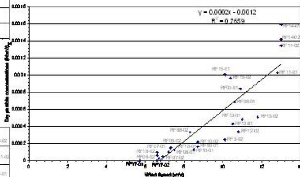
Dry particle concentration as a function of radius larger than 5 micron versus Wind Speed Circle 01 and 02
