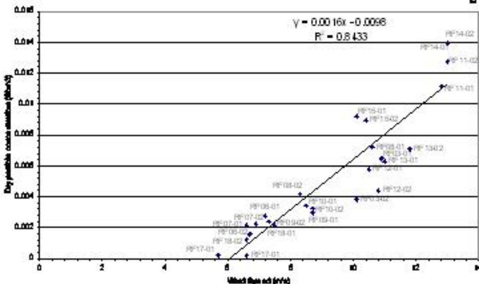
Dry particle concentration as a function of radius larger than 3um versus Wind Speed Circle 01 and 02
