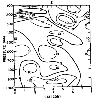
Fig. 4.37 Apparent vorticity source Z ( 10^{-11} \text{ s}^{-2} ) in the A/B scale area from Stevens.
