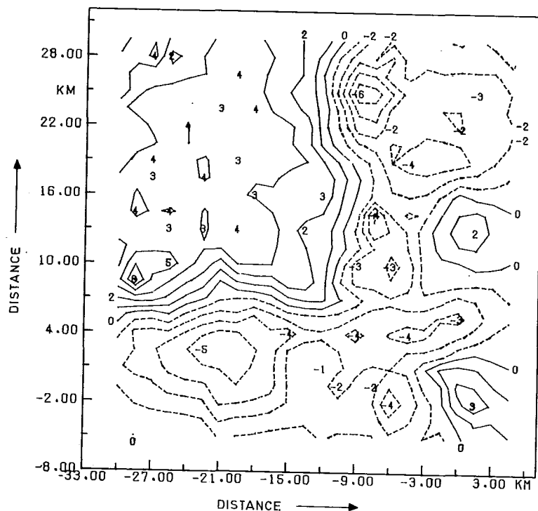
Figure 7.6 - Deviation from mean potential temperature on the density surface \sigma_t = 23.60 in the GATE C-scale area from undulating bathfish data during Phase III. The distances are measured relative to an origin moving with the mean current at the surface. Units are given in 10^{-2} degrees Kelvin (after Woods et al., 1981).
