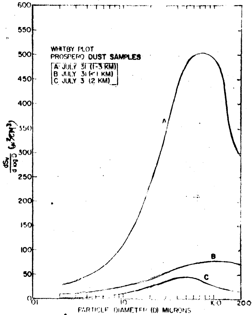
Fig11.33 Whitby plot for composite dust spectra measured with a Royco 220 aerosol spectrometer aboard the NOAA DC-6 aircraft near Sal on July 31 (spectra A and B) and south of Dakar on July 3 (spectrum C). Flight altitudes are listed in the inset
