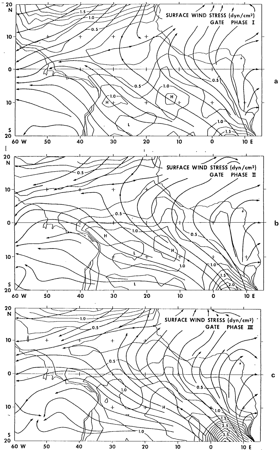
Figure 3.8 - Mean fields of total surface wind stress ( \text{dyn}\cdot\text{cm}^{-2} ) for (a) Phase I, (b) Phase II and (c) Phase III of GATE.
