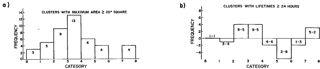
Fig. 4.21 Frequency distribution of (a) the mean location of the center of each cloud cluster versus wave phase category for all clusters with maximum area > (20^\circ)^2 and (b) the excess (positive ordinate values) or depict (negative ordinate values) of cluster genesis over cluster decay by wave phase category for clusters with lifetimes > 24 h.
