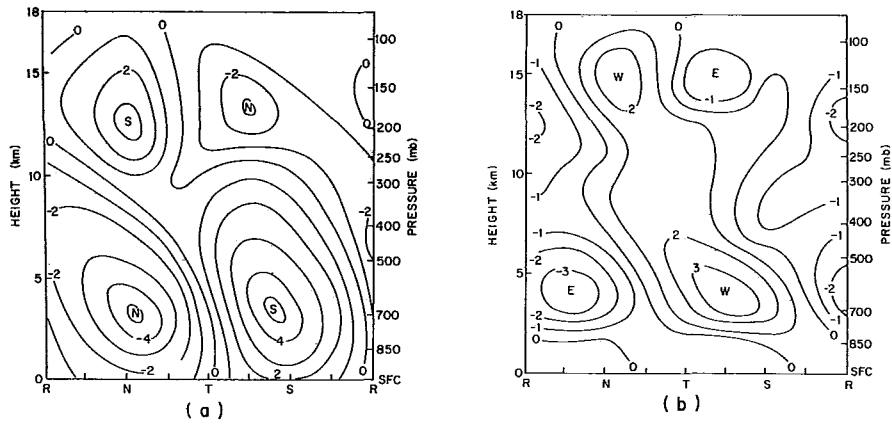
Fig. 4.10 Vertical cross sections along reference latitude. R,N,T,S refer to ridge, north wind, trough, south wind sectors of the wave. (a) Meridional wind deviation ( \text{m s}^{-1} ); (b) zonal wind deviation ( \text{m s}^{-1} ). (Fig. 4.10 continued , next page.)
