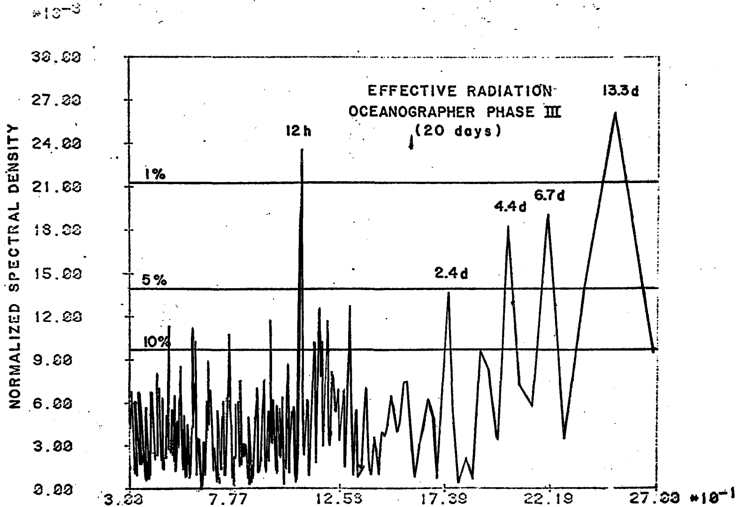
Fig.11.5 - Spectral density of the flux P(\lambda) . (according to Galindo, paper at Kiev Conference, 1980)
