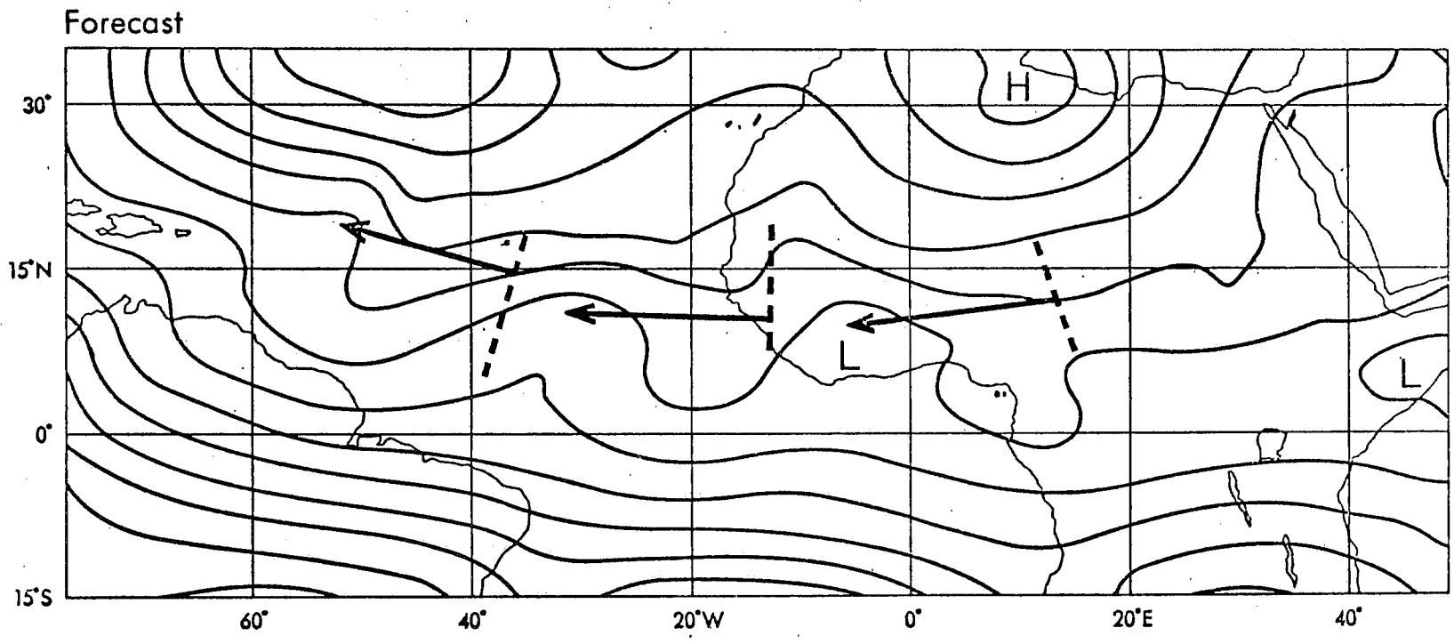
Figure 6.8(b): As Fig. 6.8(a) but for 72 hour forecast with MO tropical model. Arrows show analysed trough movements over the 72 hours.
