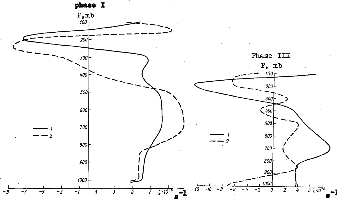
Figure 8.8 - Relative vorticity for Phases I and III of the A/B ship array observations. 1) for Class B and 2) for Class C.
